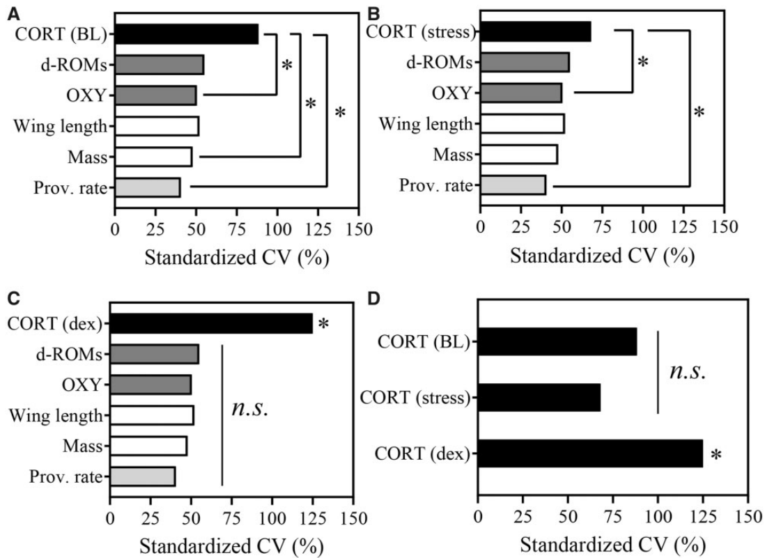
Fig. 1 Pairwise comparisons of within-population variability between baseline CORT (A), stress-induced CORT (B), and post-dex CORT (C) and other traits, plus the three CORT measures compared with one another (D). The plotted value is the coefficient of variation (CV) computed after each variable was rescaled to fit minimum = 0 and maximum = 100. Statistically significant comparisons ( P < 0.05 ) are denoted with a bracket and asterisk (*) or a single asterisk above the different trait while statistically similar variables are denoted n.s. All models accounted for within-individual CV (measurement error or within-individual variation), though it is nonetheless uncorrelated with population CV (B; R^2 = 0.10 , P = 0.487 ). Note that each panel shows combinations of the same data, but we separated each set of model comparisons into its own panel for clarity.
