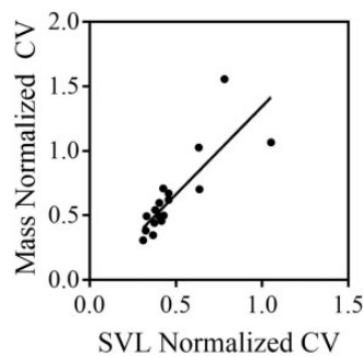
Fig. 3 Among 17 Anolis lizard species (each point = 1 species), the only traits exhibiting correlated variability are SVL and mass ( F_{1,12} = 41.6 , P = 0.0002 ). The best-fit line generated from PGLS is shown.
